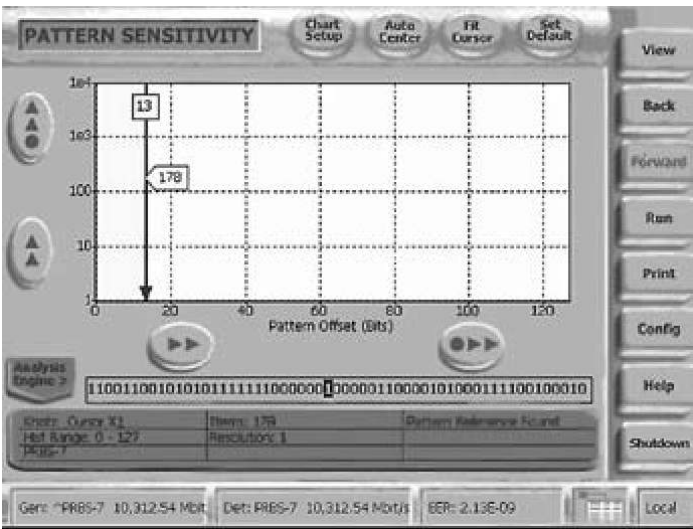
The Pattern Sensitivity view is a powerful way of examining whether error events are pattern related. It shows which pattern sequences are the most problematic, and operates on PRBS and user-defined patterns.
